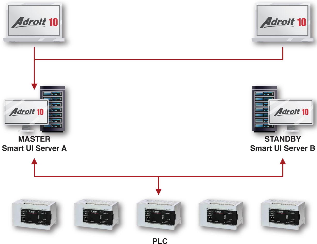
Figure 3 Active Clustering
