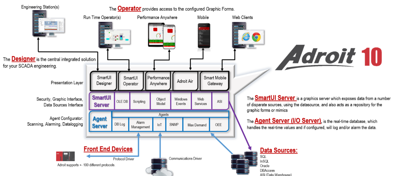
Figure 6 Adroit - Definition of Components
