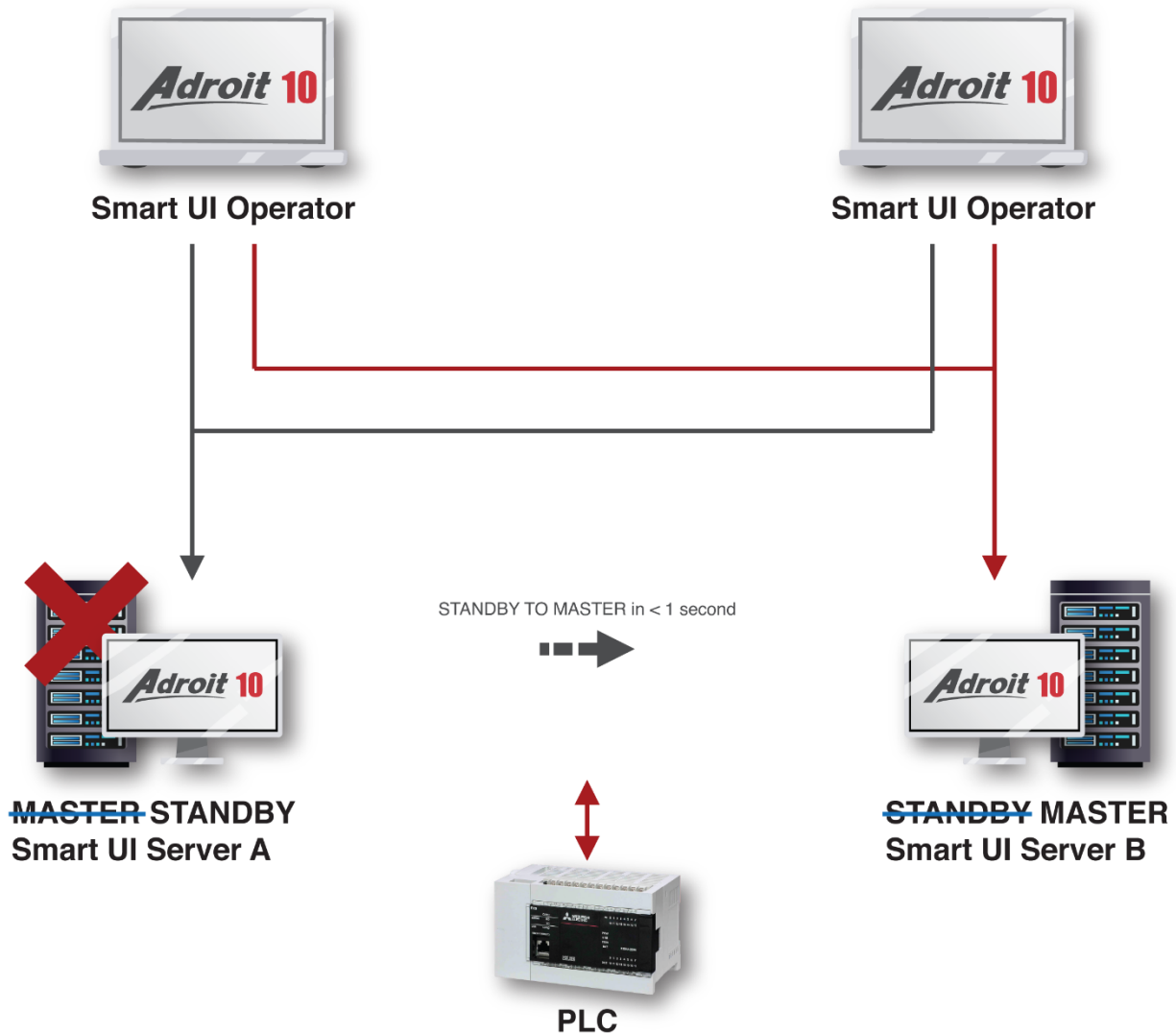
Figure 8 Adroit in a stand-alone or distributed system
