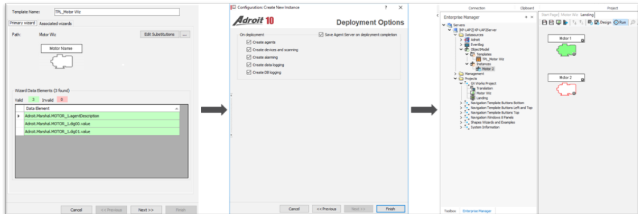
Figure 4 Object Model
